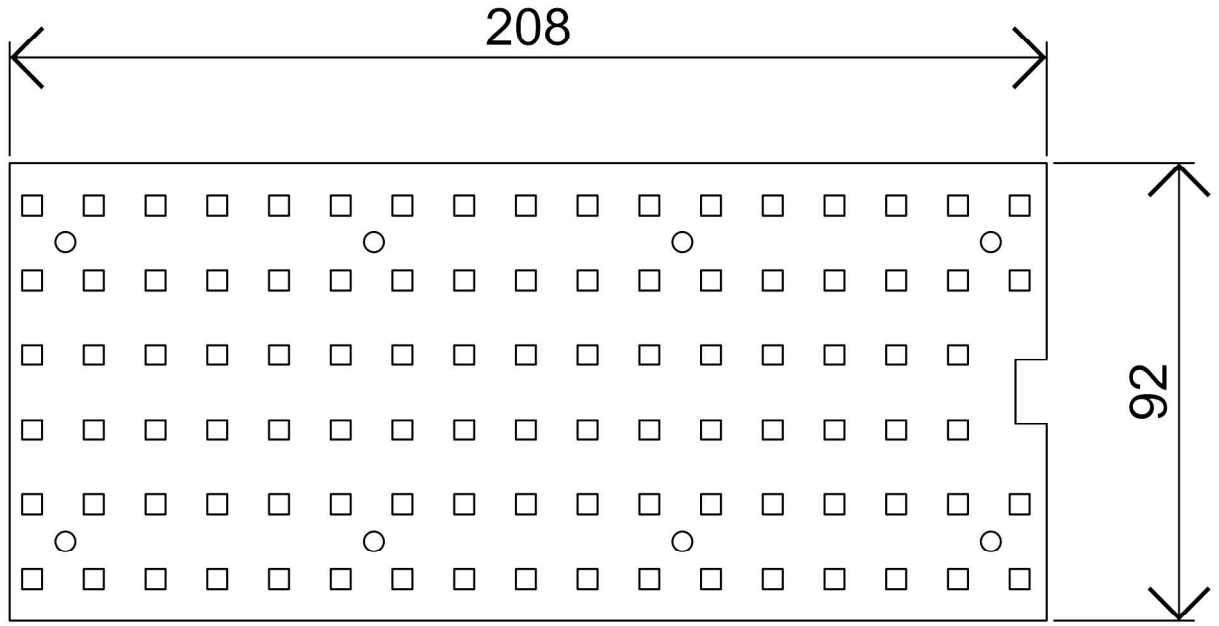
铝基板:92mm*208*T1.2mm
